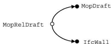
Fig. 4. Creation of a new link between a semantic building element and a new semantic element.
