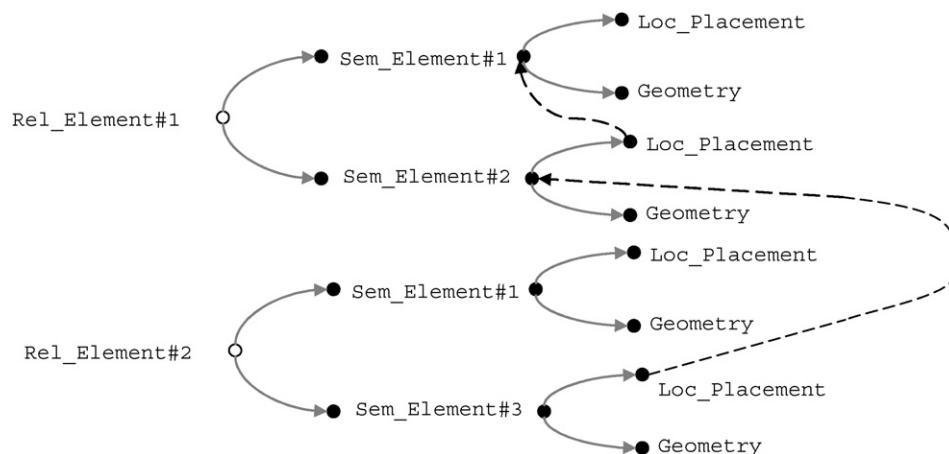
Fig. 2. Example of direct links and indirect links between semantic elements.
