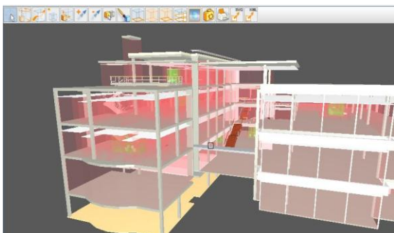
Fig. 7. Structural view of a building. This view is required for structure engineers. The corresponding graph provides all elements needed to make structure calculations.
