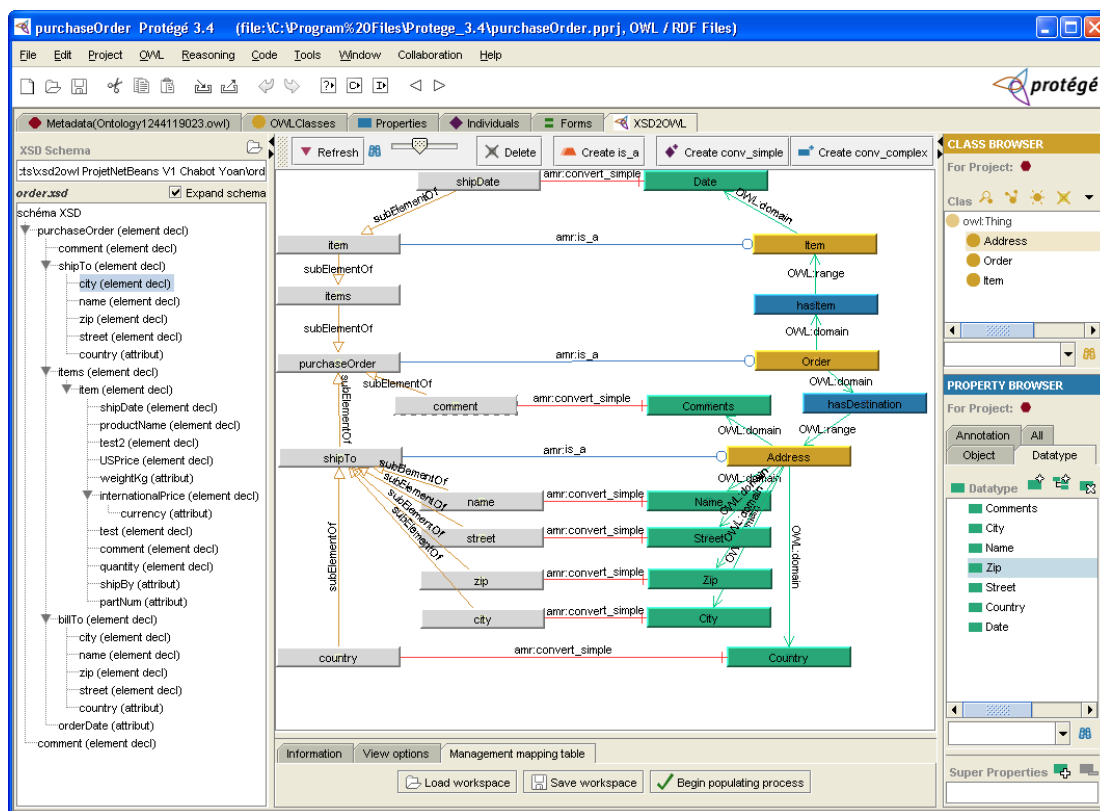
Fig. 1. Snapshot of the GXSD2OWL plug-in.
